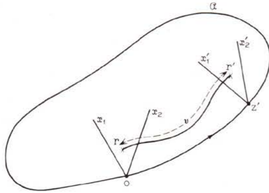
Fig. 1—Optical axis of a ring type resonator. $\mathcal{U}$ denotes the point characteristic of the system included between two transverse planes, $z = 0$ and $z = z'$.
